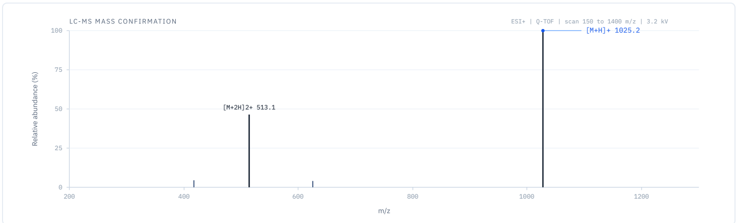
Figure 3. LC-MS mass confirmation (electrospray positive mode). Base peak [M+H] + at m/z 1025.2 with [M+2H] 2+ at 513.1, consistent with the 1024.2 Da mass of Melanotan II (MT-2) and confirming identity.
