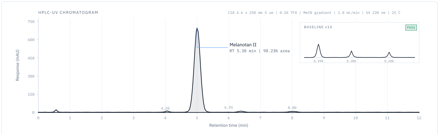
Figure 2. Representative reversed-phase HPLC-UV chromatogram (Conformity unit V1, 98.23% main-peak area, near the batch mean of 98.26%). Trace related substances are shown magnified 10x in the inset. A sharp, symmetric principal peak with a low related-substance burden is consistent with high chromatographic purity.
