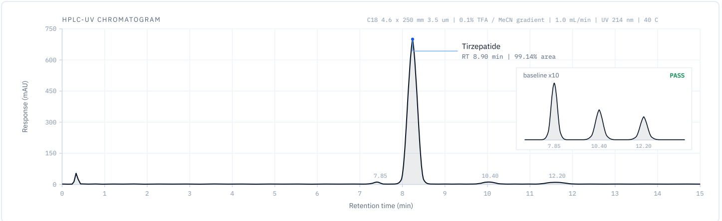
Figure 2. Representative reversed-phase HPLC-UV chromatogram (Conformity unit V1, 99.14% main-peak area, near the batch mean of 99.15%). Trace related substances are shown magnified 10x in the inset. A sharp, symmetric principal peak with a low related-substance burden is consistent with high chromatographic purity.
